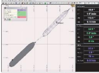
Tandem Mooring
